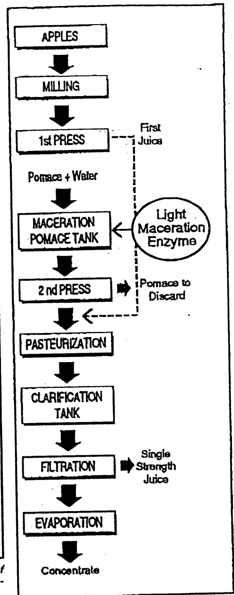
Fig. 3—Flow Process for the production of clear apple juice demonstrating light maceration with enzyme treatment of the pomace
