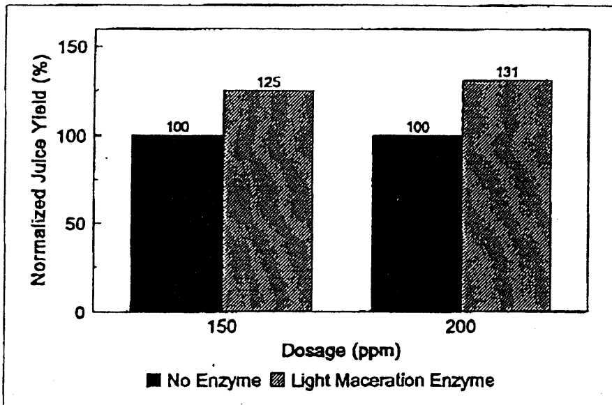
Fig. 5—Comparison of Juice Yields from apple pomace that received no enzyme treatment (black bar) and apple pomace that was enzyme treated with the light maceration enzyme (slashed bar) for 1.5 hours at 25°C, then pressed. Normalized yields were calculated as the percent (w/w) of juice obtained as related to the amount of apples pressed
