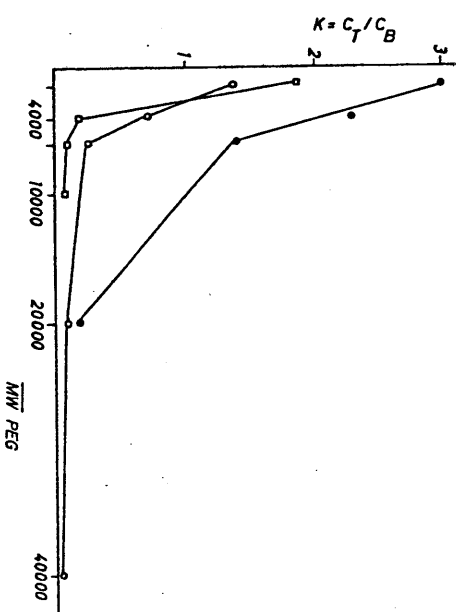
Fig. 2. Influence of the average molecular weight of polyethylene glycol on the partition of three enzymes: ○—○ pullulanase from Klebsiella pneumoniae (12% w/w polyethylene glycol, 1% w/w dextran T 500, 10 mM sodium phosphate, pH 7.5); □—□ 1,4- \alpha -glucan phosphorylase from K. pneumoniae (9.3% w/w polyethylene glycol, 7% w/w dextran T 500, 50 mM potassium phosphate, pH 7.8); ●—● leucyl-tRNA synthetase from Escherichia coli (9.2% w/v polyethylene glycol, 6.3% w/v dextran T 2000, 73 mM potassium phosphate, pH 7.0).
